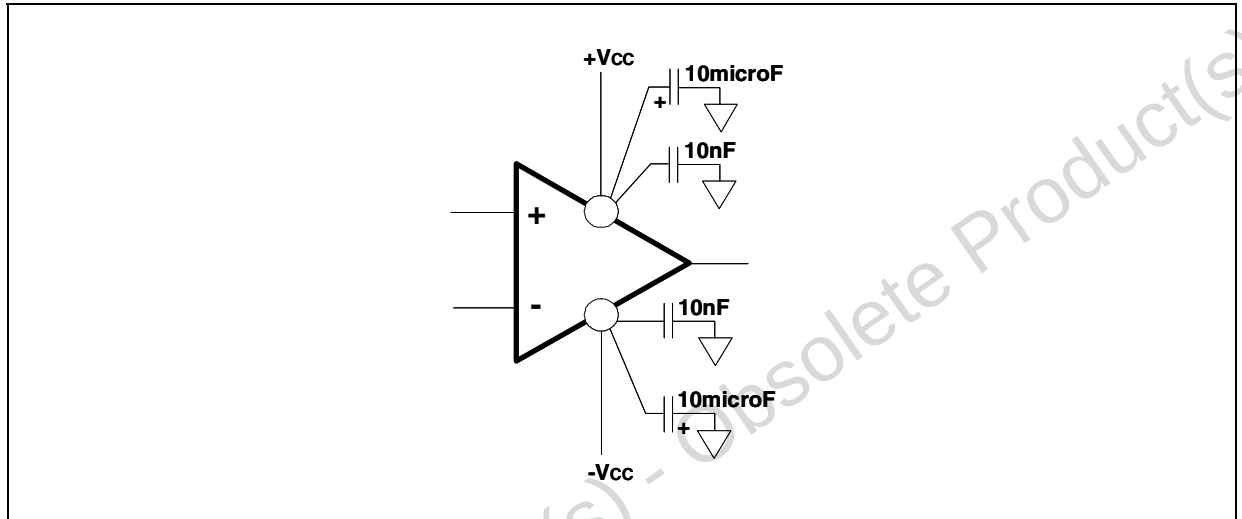
Figure 26: Circuit for power supply bypassing
